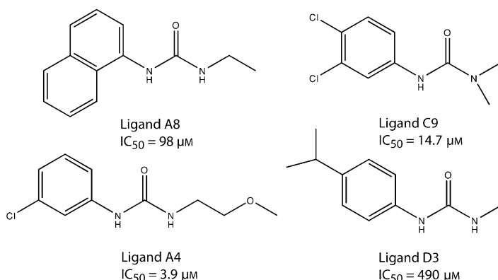
Scheme 2. sEH binding ligands that share the central urea moiety. [13]
